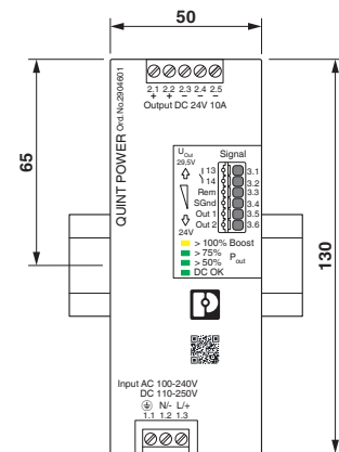
Schematic diagram
